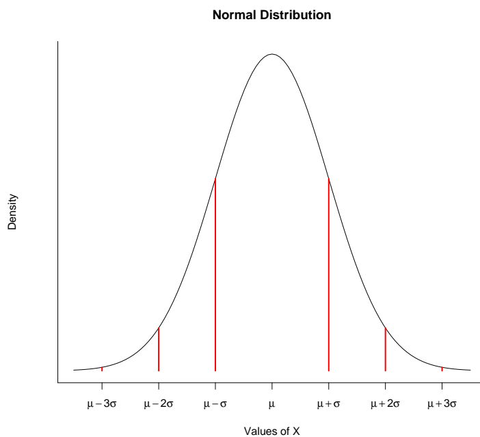
Figure 11: Normal distribution.
