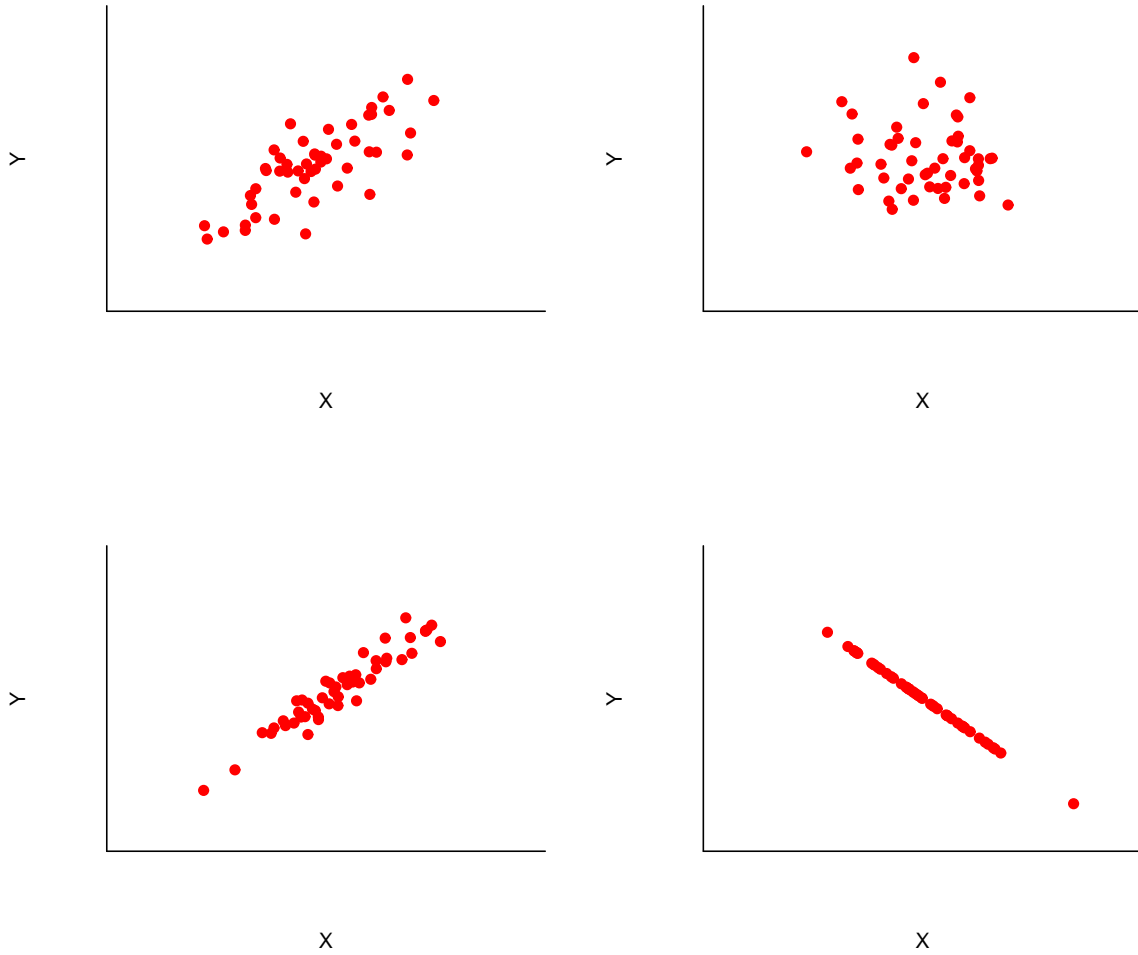
Figure 21: Example scatterplots
