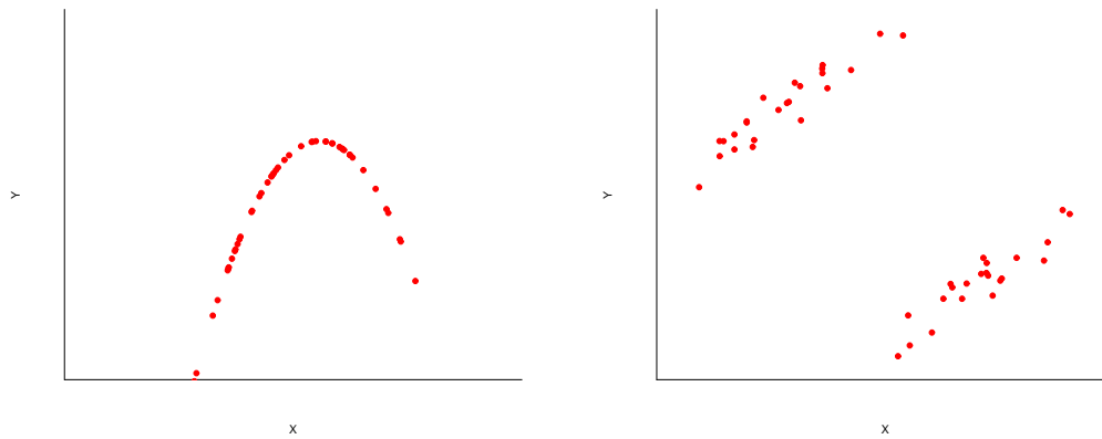
Figure 22: Example scatterplots
